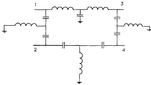
Fig. 2. Schematic diagram of a balun
