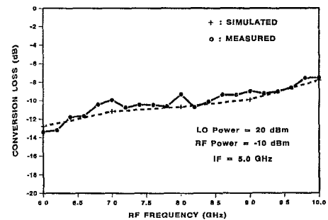
Fig. 4. Measured and simulated conversion loss versus RF frequency.
